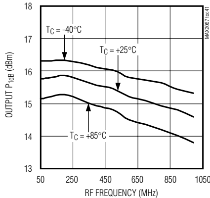
OUTPUT P 1dB vs. RF FREQUENCY (LOW-CURRENT MODE)
